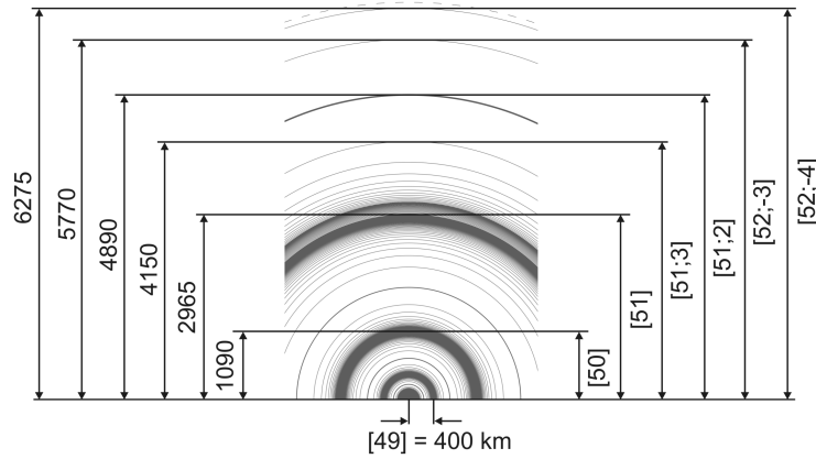
Figure 9: The Fundamental Field with equipotential surfaces of proton stability in the linear 2D-projection for k = 1 in the interval [49] \dots [52;-4] . Radius in km (left side). The dotted line at the top indicates the Earth surface that coincides with the equipotential surface E[44;4] = 6372 km of electron stability.
