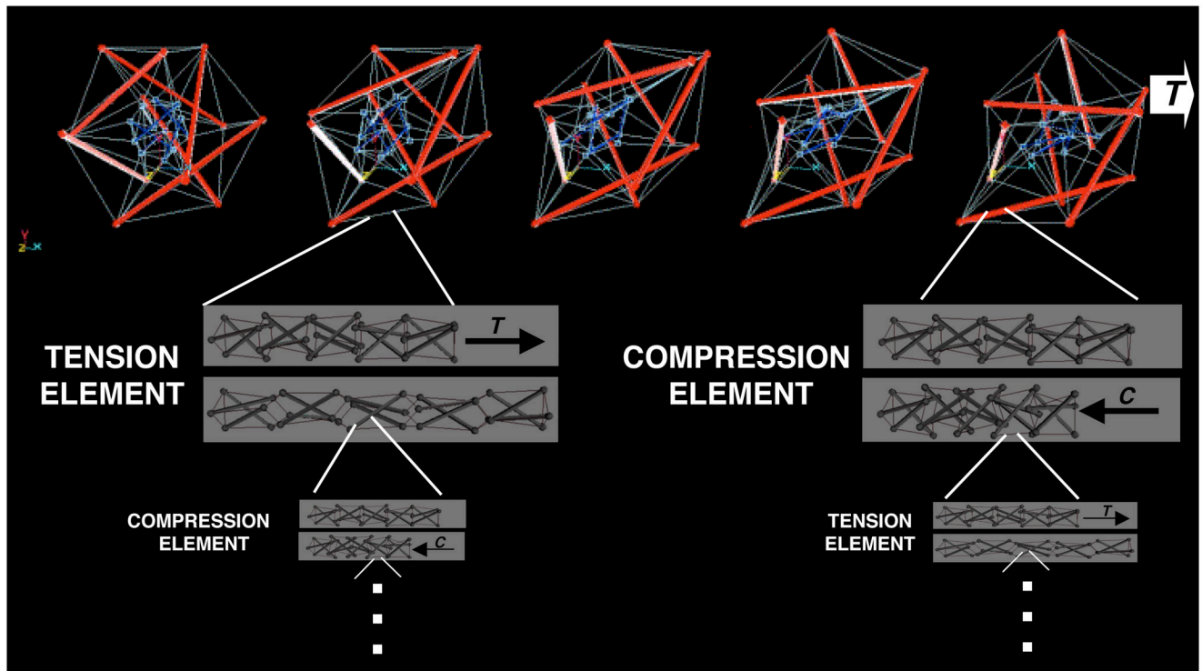
Fig. 5. Computer models depicting multiscale structural rearrangements with a prestressed tensegrity hierarchy
