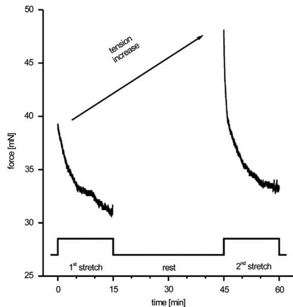
Figure 2 An example of the strain hardening effect of repeated isometric stretches. Reaction of a piece of mouse lumbar fascia in response to repeated strain application. A 4% strain is applied for 15 min, followed by 30 min of rest at zero strain. Lastly the tissue is stretched again. Tissue tension is measured at all times with an electronic force transducer. Note the increase in tension between the first and second stretch indicating an increase in tissue stiffness and resembling the strain hardening phenomenon.
