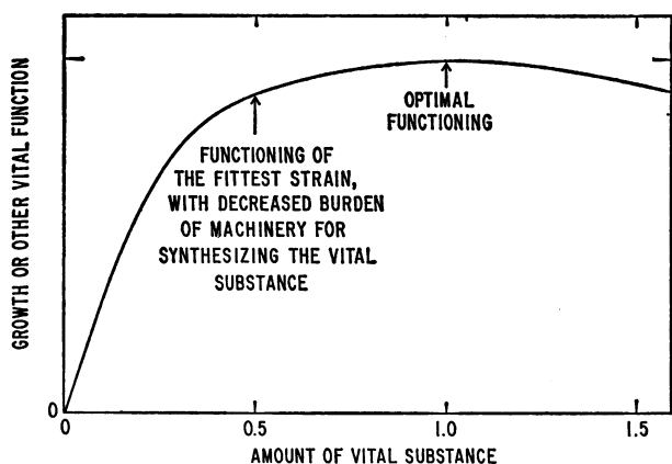
Fig. 1 (left). Diagrammatic representation of growth rate or other vital property of an organism as function of the concentration of vital substance in the organism, showing the concentration at which the differential advantage of an increased amount of vital substance is just balanced by the differential disadvantage resulting from an increased amount of machinery for synthesis, and the concentration that gives optimum functioning without consideration of the burden of the machinery for synthesis. Fig. 2 (right). The observed rate of growth of a pyridoxine-requiring Neurospora mutant (Beadle and Tatum, 1941), as function of the concentration of pyridoxine in the medium.
