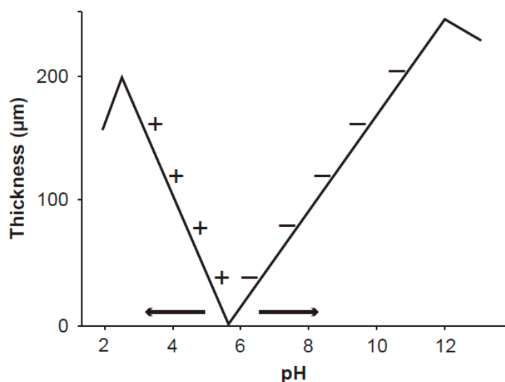
Figure 1. Schematic visualization of the thickness of the exclusion zone versus pH factor at the surface of polyvinyl alcohol gel [14]. The gel was stored in pure water at pH 5.7. The signs + and – denote positively and negatively charged particles suspended in aqueous solution at different pH and excluded from the exclusion zone. The exclusion zone is formed by the static electric field emanating from the gel surface charge. The measured curves are important for understanding the ordered water layers around mitochondria. As the inner membrane potential of mitochondria depends on the level of oxidative metabolism ( i.e. , on the intensity of the static electric field), the working point shifts along the curve and very likely even the point of zero thickness may move as shown by the arrows. The shifts of the working point along the pH axis seem to explain Warburg’s “more structure” in normal cells.
