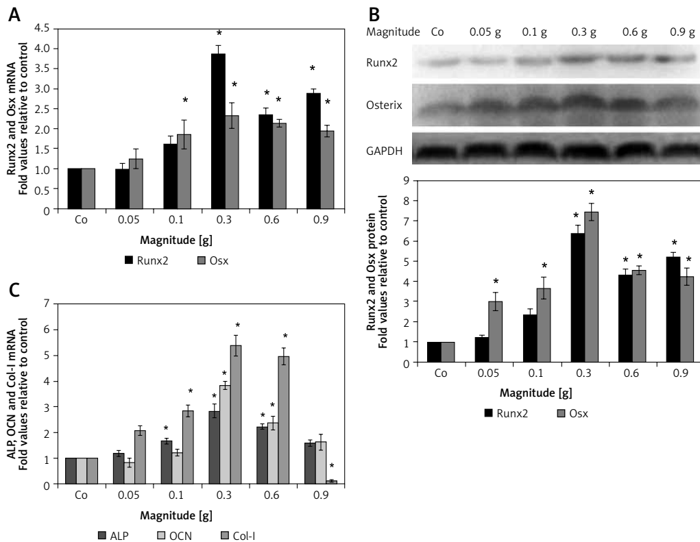
Figure 2. The effect of mechanical vibration at different magnitudes on osteogenic gene and protein expression in hPDLSCs. Quantitative PCR results indicate that Runx2 and osterix (Osx) mRNA levels were upregulated by mechanical vibration at 0.1–0.9 g magnitude, as compared to control cells (Co) (A); the mRNA expression levels of ALP, OCN, and Col-1 were in a common growing trend towards a significant peak at 0.3 g, then decreased to a minimum at 0.9 g (B); Runx2 and osterix (Osx) protein expression levels increased with increasing magnitude, peaking at a magnitude of 0.3 g compared to control (C)
