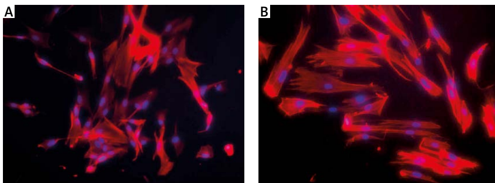
Figure 4. Change in cytoskeleton of hPDLSCs in response to mechanical vibration. Compared with the static control group (A), the F-actin stress fibers of hPDLSCs became thicker and clearer following vibration stimulation (B)
