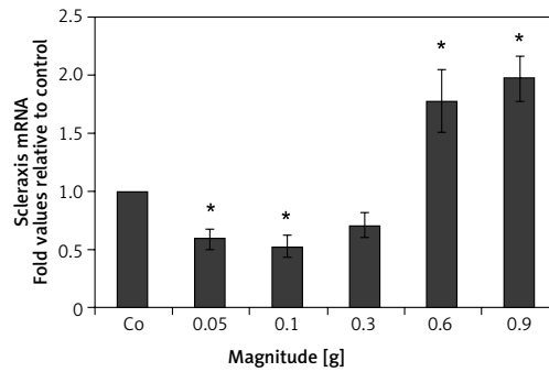
Figure 3. The effect of mechanical vibration at different magnitudes on tenogenic gene expression in hPDLSCs. Quantitative PCR results indicate that the mRNA expression level of Scleraxis, a tendon specific transcription factor, decreased at 0.05 g, 0.1 g, and 0.3 g, and significantly increased at 0.6 g and 0.9 g, with a peak increase at 0.9 g
