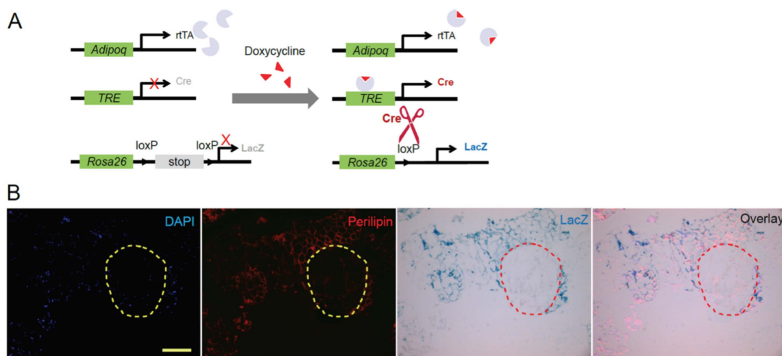
Fig. 1. Detection of de novo adipogenesis using AdipoChaser mice. (A) Schematic graph of the AdipoChaser system. Adiponectin-rTA (Adipoq-rTA), TRE-Cre and Rosa26-loxP-stop-loxP-lacZ triple transgenic mouse is hereby called the AdipoChaser mouse. It constitutively expresses rTA in mature adipocytes but only expresses Cre when doxycycline (dox) is supplemented. The Cre will subsequently recombine the loxP sites and remove the stop cassette to allow expression of LacZ. The LacZ expression will persist even after removal of dox. But new adipocytes emerging from non-adiponectin expressing progenitor or stem cells after doxycycline removal will not express LacZ. LacZ reacts with X-gal (5-bromo-4-chloro-3-indolyl- \beta -D-galactopyranoside) and develops a dark blue color. So existing mature adipocytes will be labeled blue after dox supplementation, and any new adipocytes emerging after removal of dox will not be labeled. (B) Representative \beta -gal (blue) and Perilipin1 (red) staining of subcutaneous white adipose tissue in AdipoChaser mouse 6 weeks after Juvederm injection. Nuclei are counterstained with DAPI (blue). The circle indicates the boundary of Juvederm and adipose tissue. Scale bar: 250 \mu m.
