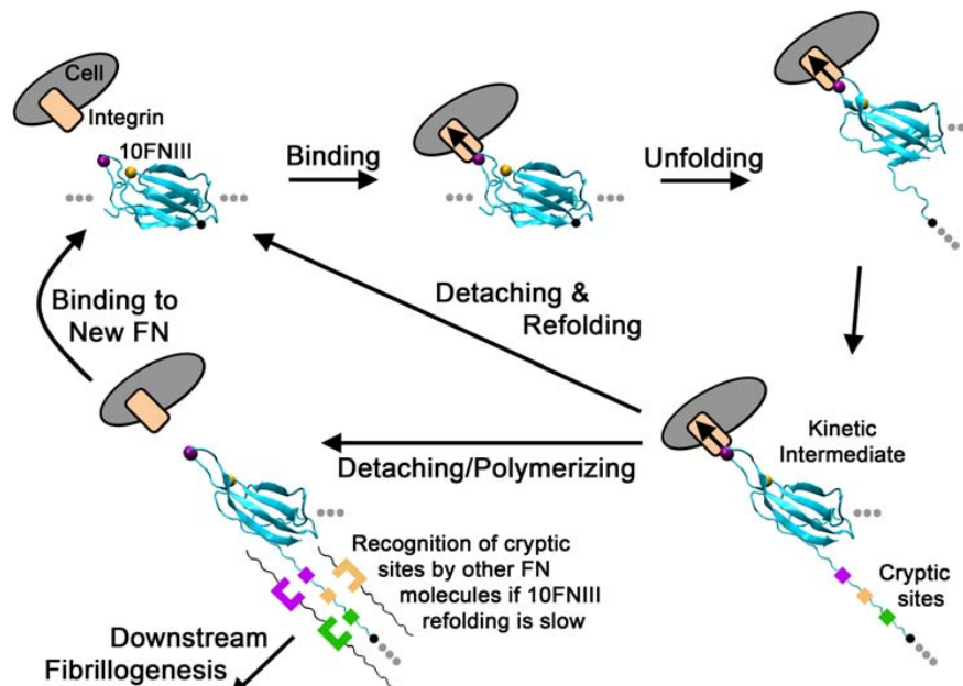
Figure 8. Cell-mediated Fibrillogenesis. The proposed model involves the formation of a partially unfolded intermediate during cell-traction mediated unfolding. Potential cryptic sites may exist in this partially unfolded structure that promote FN aggregation and fibrillogenesis. Subsequent unfolding past this intermediate induces a crucial arginine at a secondary binding site to move to a position far from the RGD loop. This frees the cell and enables it to reattach to another FN molecule to propagate the process. If 10FNIII refolding is relatively slow, then unfolded portions of this domain can make contacts with other FN molecules.
