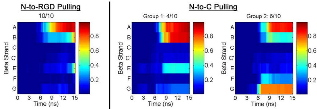
Figure 4. Solvent Accessibility Factor of Each \beta -strand During the Early Stages of Unfolding. The color scale (right), ranging between 0 and 1, represents the degree of solvent exposure of the \beta -strand (labeled A through G, left) for time \leq 15 ns. With this scaling, \beta -strands in the initial structures all have f=0 , while fully exposed strands have f=1 . doi:10.1371/journal.pone.0002373.g004
