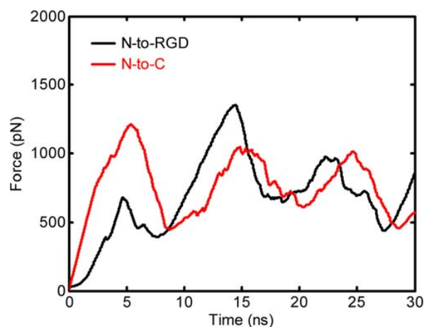
Figure 2. Extension Force Associated with Unfolding 10FNIII Along Either Axis. Averaging across each of the ten simulations along the N-to-RGD (black) or N-to-C (red) axis shows that the general properties of the force profiles are similar. doi:10.1371/journal.pone.0002373.g002
