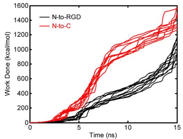
Figure 7. Calculation of the Work Needed to Partially Unfold 10FNIII Along Either Axis. Data for each of the 10 simulations pulled along N-to-RGD (black) and N-to-C (red) are shown for the first 15 ns. doi:10.1371/journal.pone.0002373.g007
