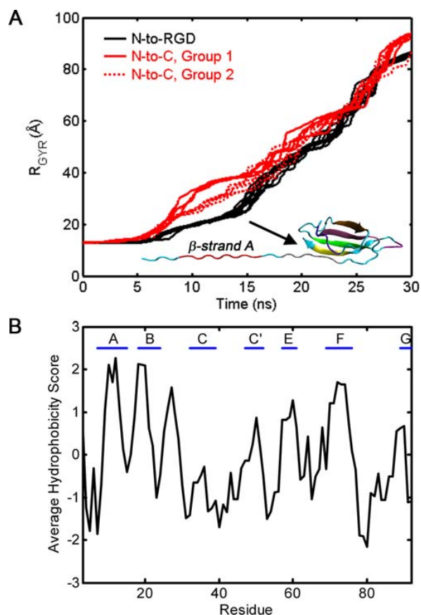
Figure 3. Different Unfolding Pathways for 10FNIII. (A) Backbone radius of gyration as a function of time for N-to-RGD (black) and N-to-C (red) pulling. The mass weighted radius of gyration is calculated for the backbone atoms (N, H, C \alpha , C, and O atoms) for all time points along the pulling trajectory. For N-to-C pulling, two groups of unfolding profiles are readily identified – red solid lines represent group 1, and red dotted lines represent group 2. Unfolding in group 1 shows larger values of extension during intermediate times. A representative structure from the pulling simulation that corresponds to the kinetic intermediate in the N-to-RGD force profile is shown (inset). The \beta -strands are colored as shown in Figure 1A with \beta -strand A labeled for clarity. (B) Kyte-Doolittle hydrophobicity values for \beta -strands in 10FNIII. With a window size of five, the Kyte-Doolittle hydrophobicity scores are computed for the 10FNIII amino acid sequence. Residue definitions for the \beta -strands defined in (A) are labeled above. doi:10.1371/journal.pone.0002373.g003
