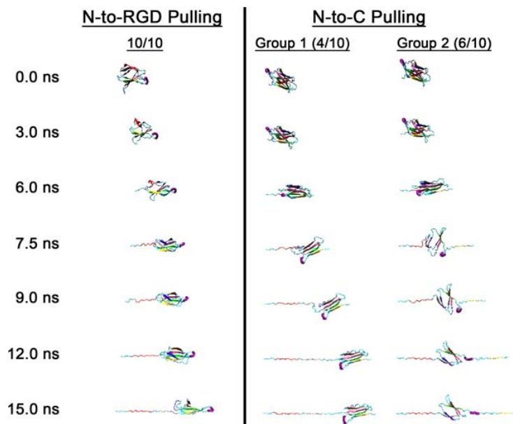
Figure 5. Snapshots of Early Events in the Unfolding Process (time \leq 15 ns). Unfolded structures show \beta -strand coloring corresponding to those defined in Figure 1A. The RGD loop is highlighted as a purple tube. The structures are oriented such that the N-terminal ends are on the left so that pulling of 10FNIII occurs towards the right. Unfolding as a function of time (labeled at left) is shown vertically for both N-to-RGD and N-to-C axes. doi:10.1371/journal.pone.0002373.g005
