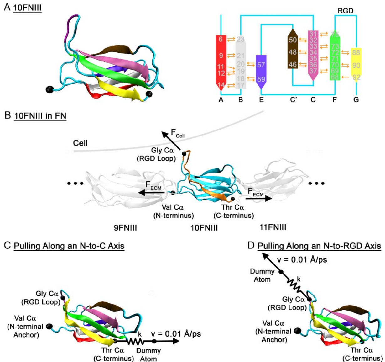
Figure 1. Local Environment of 10FNIII. (A) Crystal structure of 10FNIII. On the left is the cell-binding module of FN (type III), whose globular folded form is composed of seven \beta -strands split between two \beta -sandwich sheets. The RGD loop is highlighted as purple in the loop connecting \beta -strands F and G. N- and C- termini are labeled as black spheres. On the right is a schematic topology map of the secondary structure of 10FNIII with each \beta -strand labeled and color-coded corresponding to the crystal structure on the left. \beta -strand boundaries are adapted from the crystal structure as previously shown [17]. Residues participating in hydrogen bonds (orange arrows pointing in the direction from hydrogen bond donor to acceptor) are labeled in gray. Hydrogen bonds shown are between backbone atoms of the \beta -strand residues and are calculated for distances within 3.5 Å and angles within 120°–180° using the software VMD. (B) 10FNIII as it sits in FN. 10FNIII, adjacent to the ninth (9FNIII) and eleventh (11FNIII) type III modules, experiences two types of forces. The cell can directly apply force ( F_{CELL} ) at the RGD loop by binding through a cell-surface integrin and applying cell traction. Force can also be applied to FN indirectly through the ECM ( F_{ECM} ). F_{ECM} represents the forces generated by cells bound to remote sites in the ECM that are propagated to 10FNIII through neighboring domains bonded at the N- and C- termini. Residues C-terminal to the RGD loop (highlighted in gold) adopt a relatively extended conformation. (C) Pulling along an N-to-C axis. The protein is anchored at the C\alpha atom of the N-terminal residue (Val1416), and force is applied through a spring (with spring constant k ) attached at the pulling point by translating the free end (attached to a dummy atom) at constant velocity ( v = 0.01 Å/ps) in the defined direction. This process transmits force to the attached C\alpha atom of the C-terminal residue (Thr1509). Each \beta -strand is color-coded and labeled as in (A). (D) Pulling along an N-to-RGD axis. The C\alpha atom of the N-terminus is anchored, and the pulling force is exerted through a spring attached to the C\alpha atom of the Gly residue in the RGD tripeptide. Each \beta -strand is color-coded and labeled as in (A). doi:10.1371/journal.pone.0002373.g001
