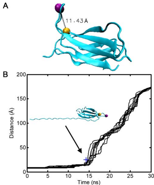
Figure 6. The Arginine Cell Detachment Trigger. (A) R1445 in the crystal structure of 10FNIII. Residues R1445 and G1494 (the central glycine in the RGD motif) are depicted as gold and magenta spheres, respectively. (B) Positioning of an essential arginine during the course of N-to-RGD unfolding. The distance between the C \alpha atoms of R1445 and G1494 is shown as a function of time for each of the ten unfolding simulations along the N-to-RGD axis. R1445 rapidly moves far from the RGD loop once the kinetic intermediate is formed (time point labeled with structure inset). doi:10.1371/journal.pone.0002373.g006
