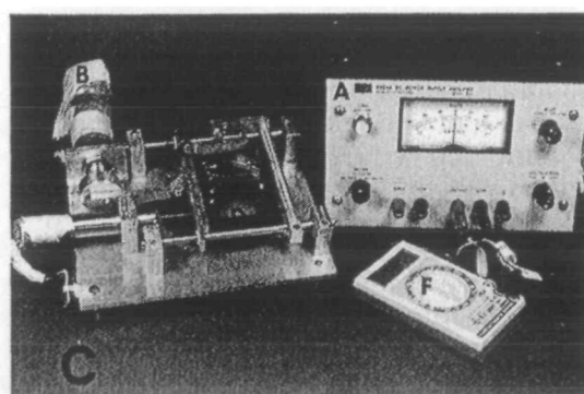
Figure 1 (a, b, c) The mechanical device is composed of an electrical transformer (A), connected to rotatory motor (B). The rotatory movement is transferred to a silicon membrane (D) through a mobile arm (C) and two episodic resin clamps attached to the membrane (E). The linear movements of the aluminum arm along two axes determined a proportionate elongation of the membrane, measured by a LVDT (Voltmeter) (F) as variation of electric potentials and transformed into millimetres with a mathematical constant.
