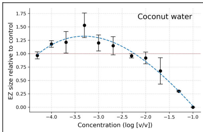
Figure 4. Effect of coconut water on exclusion zone (EZ) size. Each point represents a mean with standard deviation (n; number of experiments = 3-7).
