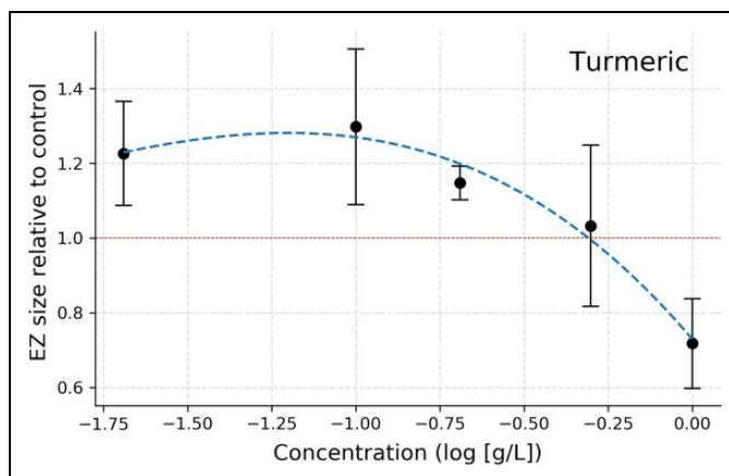
Figure 5. Effect of turmeric on exclusion zone (EZ). Each point represents a mean with standard deviation (n; number of experiments = 7-10).
